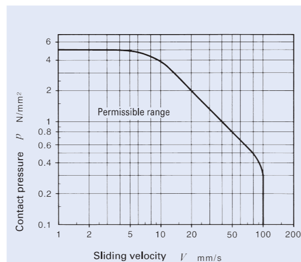
Fig. 2 pV diagram of lubrication type PILLOBALLS
